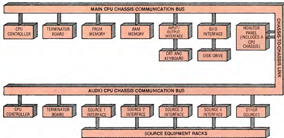
Figure 1. The architecture of a typical program automation system. Multiple microcomputers may be used, depending on the system design, to control various functions.
