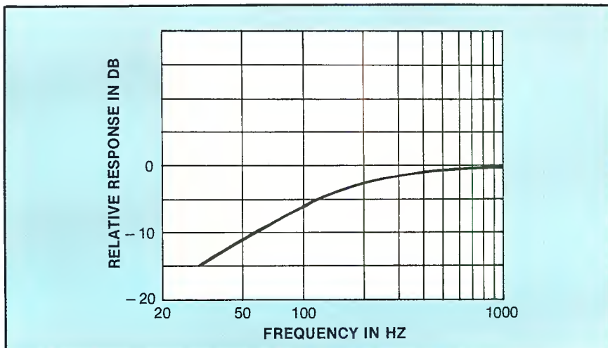
Figure 1: Frequency response curve for the low-cut filter available on each input channel.
