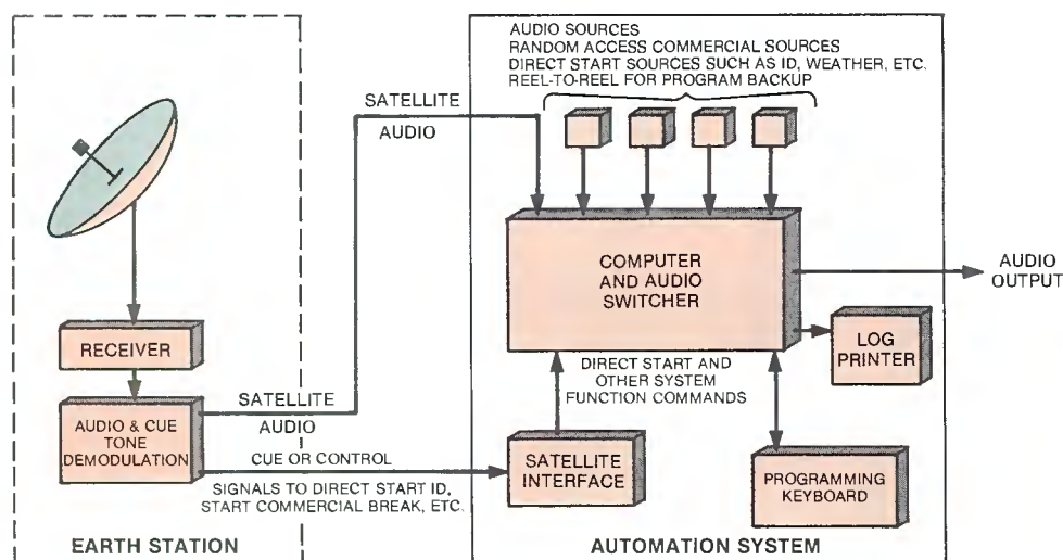
Figure 5. Typical equipment configuration of an automated station using a satellite-delivered program service.
