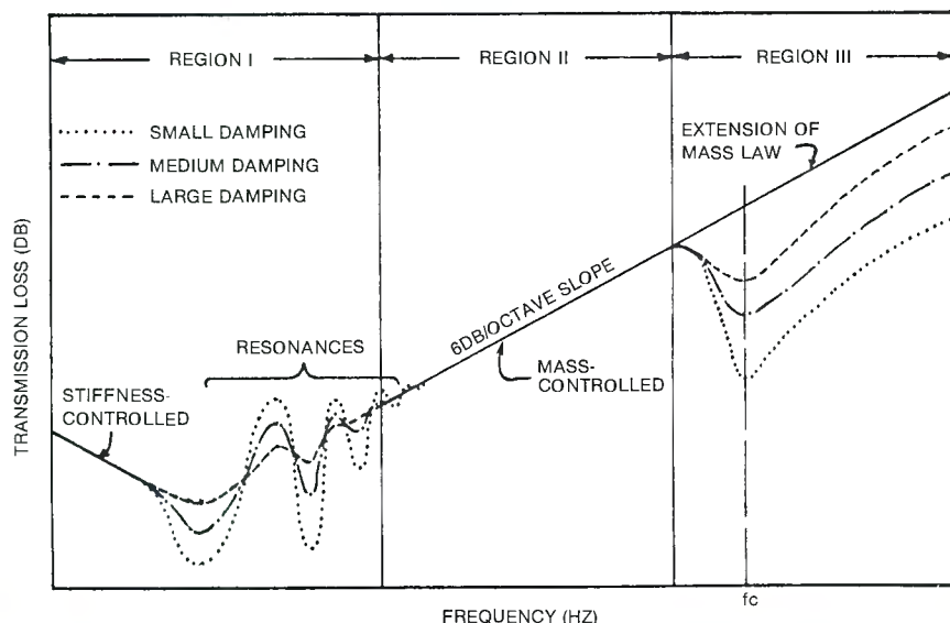
Figure 1. Sound transmission loss of typical materials.
